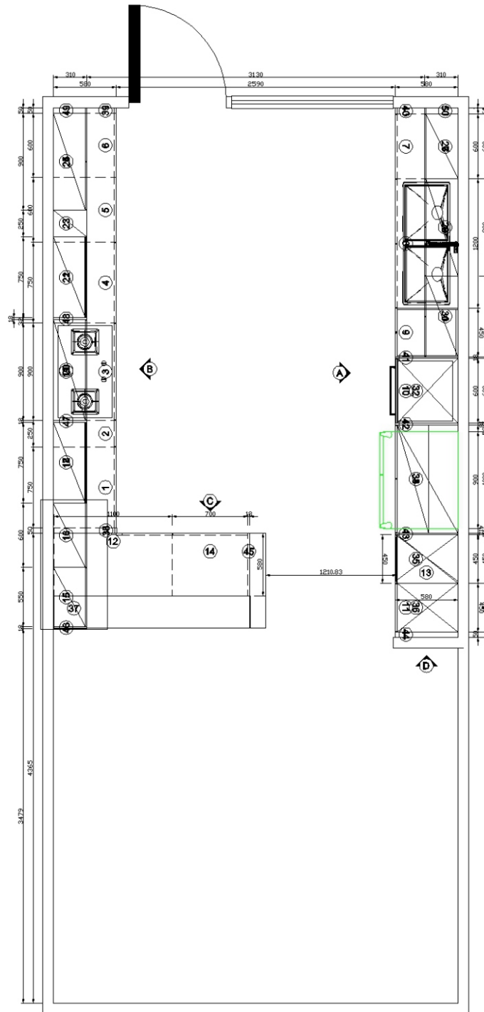
Plan drawing
