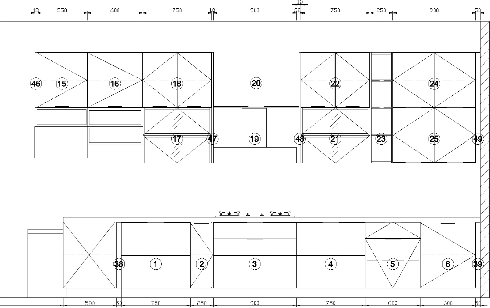
B View elevation drawing
